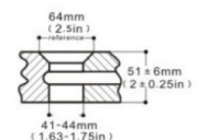
Lavatory and Bidet Outlet Detail
