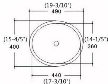
Lavatory and Bidet Outlet Detail
