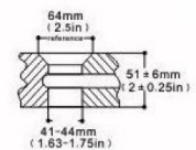
Lavatory and Bidet Outlet Detail
